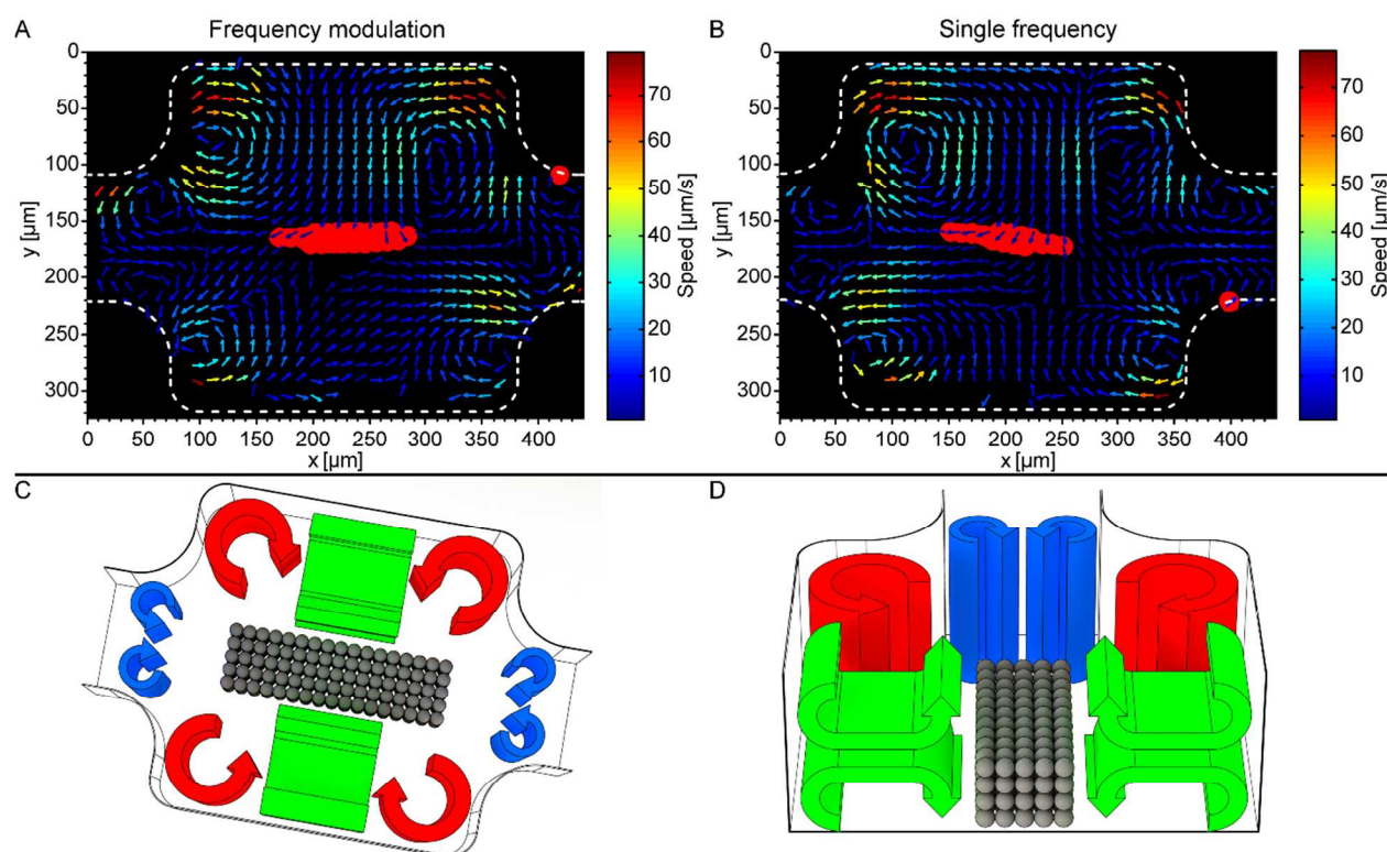
Figure 5: Quantitative (A-B) and qualitative (C-D) description of the acoustic streaming in the micro-box-cage. (A): Micro-particle-image-velocimetry (μPIV) of the acoustic streaming when implementing frequency-modulated (FM) ultrasound (2.53 MHz, span 0.1 MHz, and a rate of 1 kHz, acoustic pressure amplitude 0.87 \pm 0.02 MPa). (B): μPIV of the acoustic streaming at single frequency (SF) ultrasound (2.53 MHz and acoustic pressure amplitude 0.87 \pm 0.02 MPa). The red colored regions in (A) and (B) indicates where the larger 10 \mu\text{m} beads are trapped. (C): Sketch of the three different types of acoustic streaming in the trapping chamber: Standard Rayleigh boundary streaming (red), smaller Rayleigh streaming located at the transitions to the inlet and outlet channel of the chamber (blue), and finally vertical Rayleigh streaming (green). The qualitative description of the acoustic streaming is verified in supplementary video S1. (D): Cross section view of (C) giving a more detailed view of the vertical streaming vortices (green). The gray colored spheres in (C) and (D) represent a trapped particle aggregate.
