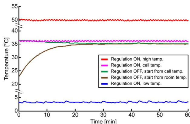
Figure 3: Demonstration of temperature control at different regulation schemes measured over a period of one hour with continuous ultrasound (frequency modulation, center frequency 2.53 MHz, span 100 kHz, rate 1 kHz, actuation voltage comparable to an acoustic pressure of 0.94 MPa). The device is tested at both low ( 3.2 \pm 0.2^\circ\text{C} , blue curve) and high ( 50 \pm 0.2^\circ\text{C} , red curve) temperatures with active temperature regulation. To ensure high cell viability the device was set to regulate a temperature < 37^\circ\text{C} , in this demonstration the “cell” temperature was 36.2 \pm 0.2^\circ\text{C} (magenta colored curve). In addition, as a control, the device was operated without active temperature regulation from room temperature (brown curve) and from “cell” temperature (green curve). As a consequence of the design of the device, the final temperature after one hour was 35.1 \pm 0.1^\circ\text{C} for the brown and green colored curves.
